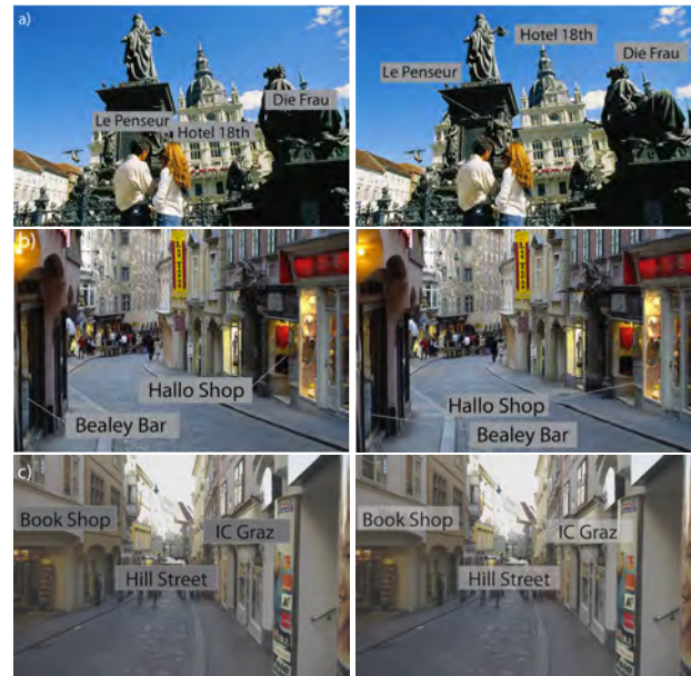
Figure 2: Illustration of three of our real world considerations (from top to bottom), bad (Left) and good (Right) examples of: (a) avoiding overlap on salient areas, (b) avoiding overlap on edges, (c) improving contrast between video image and labels.
