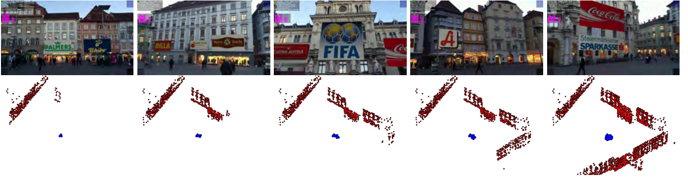
Fig. 11: Top row: Annotation results from a rotation-only sequence. Bottom row: Expanding SLAM map, while the user rotates a handheld device. The map nicely resembles the structure of the surrounding buildings.
