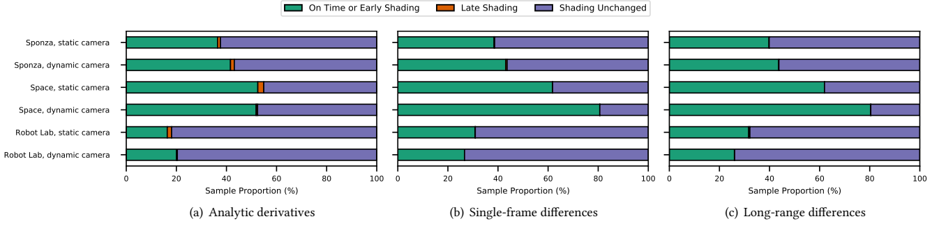
Fig. 9. Applying an image-space filter on top of the gradients strongly reduces late shading compared to Figure 7. While analytic derivatives still lead to late shading, finite differences—in both versions—effectively avoid late shading. Obviously, distributing shading predictions to neighbors increases early shading, leading to less reuse and thus less performance improvement, especially in the highly dynamic scene Space . Note that this visualization does not tell us how much reuse is possible, since we cannot distinguish by how many frames shading is early. Please see the supplementary material for the exact distribution of early and late shading.
