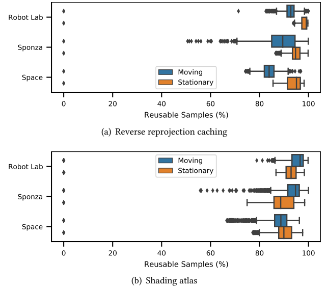
Fig. 5. We determine the possible reuse of two rendering approaches based on visibility and a color difference threshold T = 8 . (a) Reverse reprojection caching accumulates spatial sampling errors over time, especially when the camera is moving. (b) In contrast, the shading atlas reuse is independent of spatial sampling, and thus the reuse correlates better with the dynamics of the shading as shown in Figure 4. We reuse a block of the shading atlas only if all the samples within the block can be reused. Outliers at 0 are caused by the first frame of the test sequence in which all samples need to be shaded.
