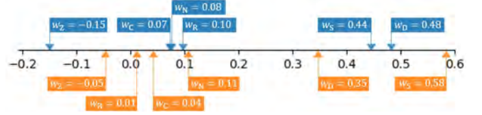
Fig. 10. Weights over all measures. We use the weighting parameters to balance the metric. We obtained the weights for color (blue) and depth (orange).
